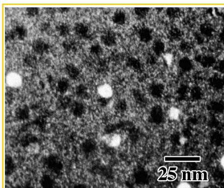
Figure 1. Dark-field TEM image of amorphous/nanocrystalline Al 90 Fe 5 Gd 5 with 10 nm nanocrystals. Here both the bright and dark spots represent nanocrystals and the gray matrix between them is amorphous Al 90 Fe 5 Gd 5 heat-treated at 150°C for 24 h. 29
