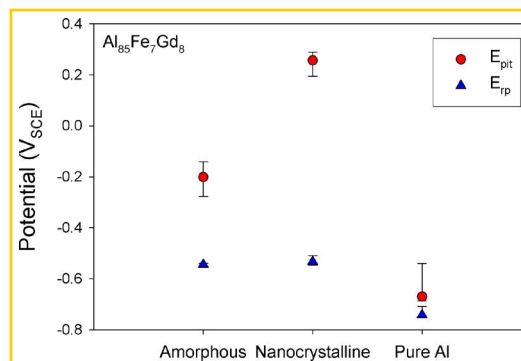
Figure 8. (Color online) Median pitting and repassivation potentials for Al_{85}Fe_7Gd_8 and pure Al in deaerated 0.6 M NaCl. Error bars represent the 25th and 75th percentile of the data. Scan rate 0.1 mV/s.
